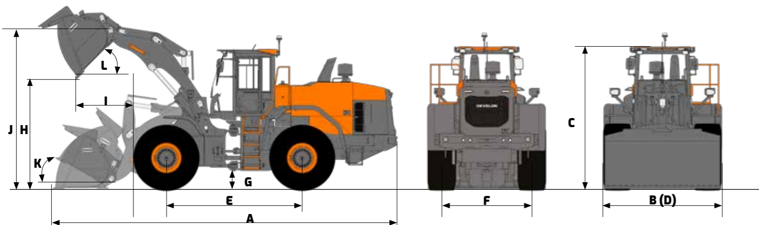
DL220-7
